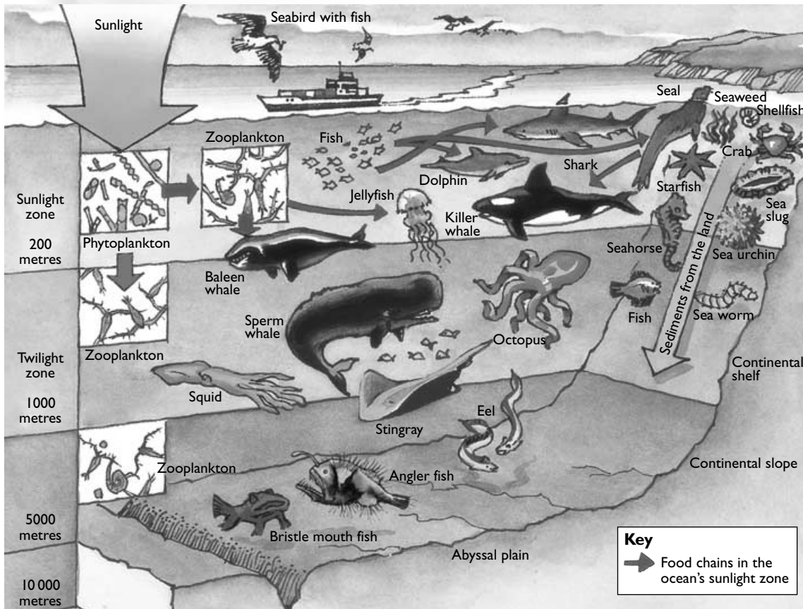
Ocean food web. This diagram is not to scale.
